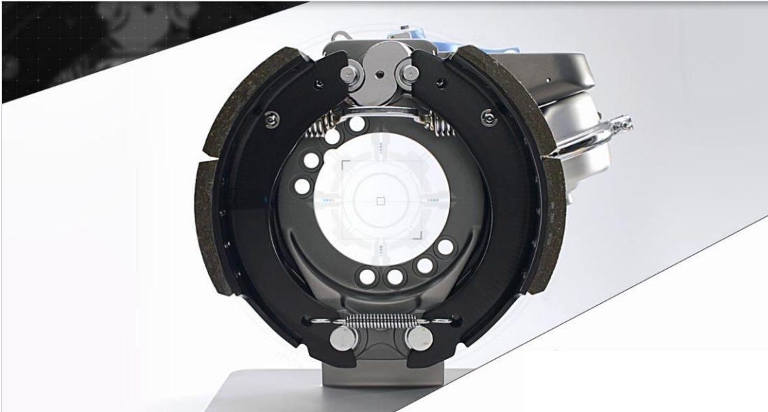
Drum Brake System for Commercial Vehicle
